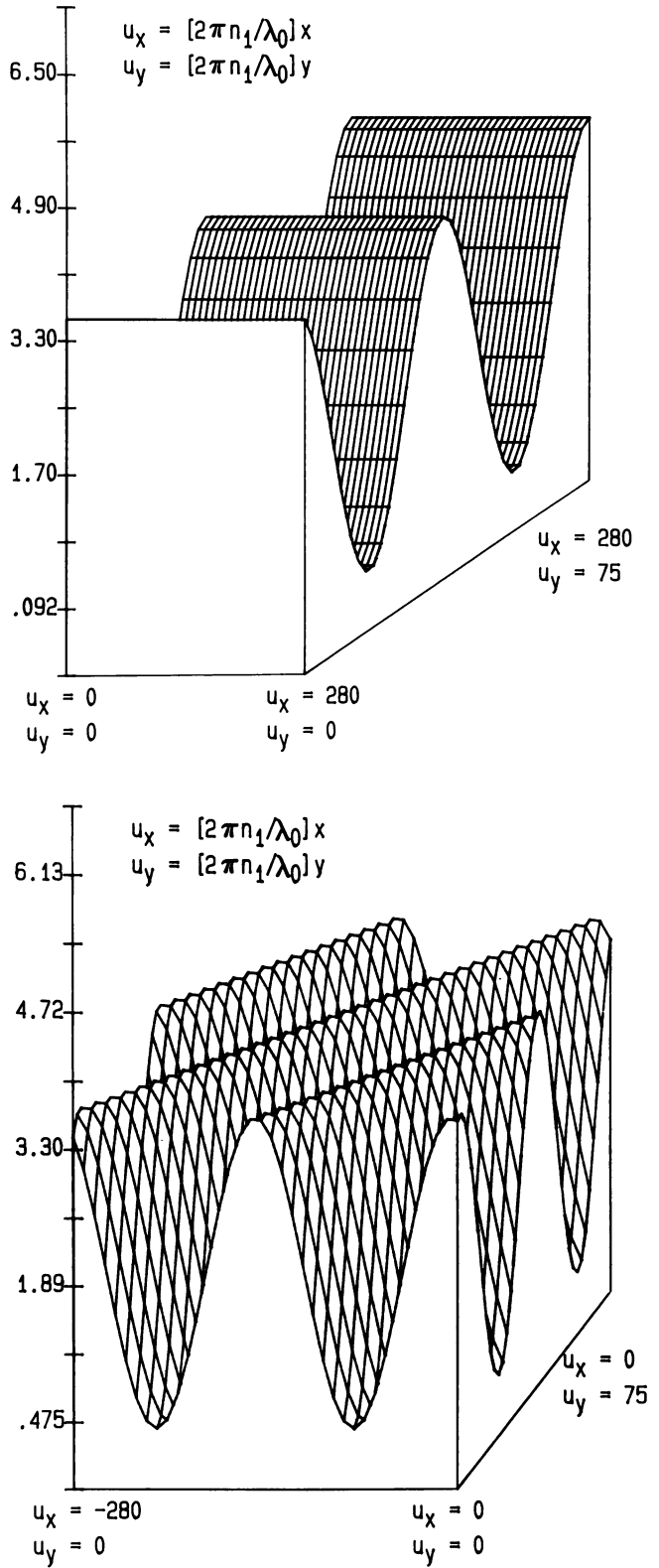
FIGURE 2 Typical interference patterns. The evanescent-wave interference patterns I(x, y) created by p-polarized beams of equal amplitude are shown for (A) \theta_1 = \theta_2 = 75^\circ and \phi = 5^\circ and (B) \theta_1 = 80^\circ , \theta_2 = 70^\circ , and \phi = 5^\circ . The primary features introduced by unequal \theta_1 and \theta_2 are reduced visibility and a rotation of the pattern. Curves were calculated using Eq. 17 with z = 0 , n_1 = 1.467 , n_2 = 1.334 , and \Delta\delta = 0^\circ .
